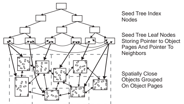
Figure 2: FLAT groups spatially close elements on object pages (rectangles at the bottom) and inserts the MBRs into the seed tree (tree structure at the top).
